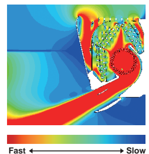
Fast ← → Slow Colours in the figure show the air speed.
